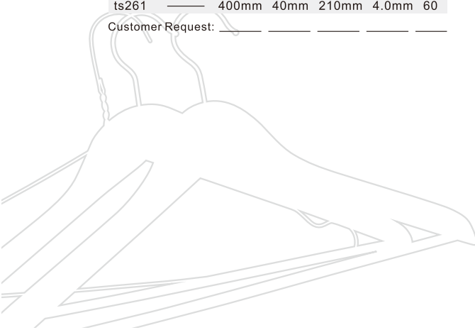
REF SHAPE ts261 — 400mm 40mm 210mm 4.0mm 60
