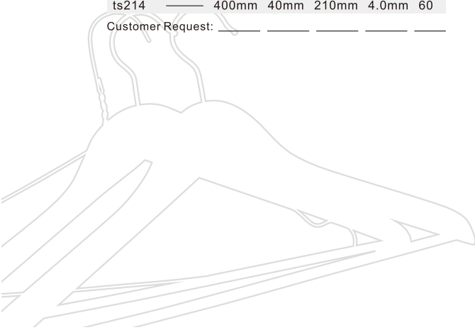
REF SHAPE ts214 — 400mm 40mm 210mm 4.0mm 60
