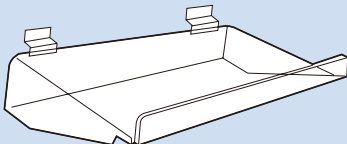
Acrylic Extra Support Shelf 3/16" clear acrylic with bent gussets for extra support. # JD870SL 8" W × 12"L # JD876SL 10" W × 16"L # JD878SL 10" W × 24"L # JD879SL 10" W × 36"L
