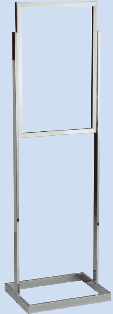
14" × 22" SIGN HOLDER Vertical frame and base are made of rectangular tubing 1/2" × 1 1/2". Base 12" × 16". Height is 53", chrome # BURT22
