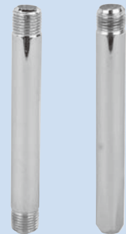
Threaded Stem Swaged Stem 3/8" Dia. rod Item Size Item Size # THR3 3" # SWE3 3" # THR6 6" # SWE6 6" # THR9 9" # SWE9 9" # THR12 12" # SWE12 12"
