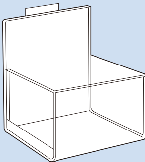
ACRYLIC HOSIERY BIN 7¾"wide × 4¾"Deep × 4½"H (Front) Non-slanting back, single bin. # S2420
